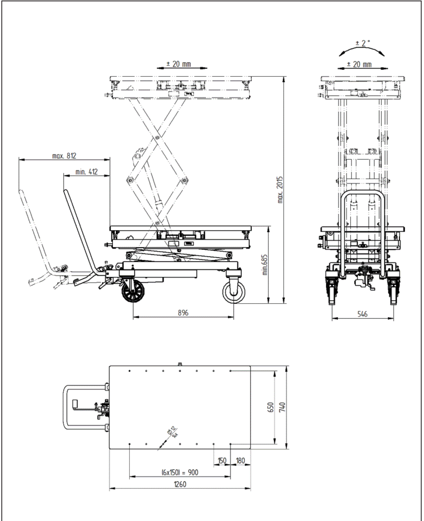
Dimension sheet Master Gear S3 1.0 with extract
